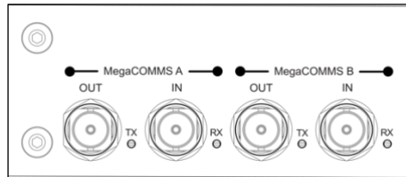
1: The CM-MD64 has two pairs of MegaCOMMS ports on BNC connectors
