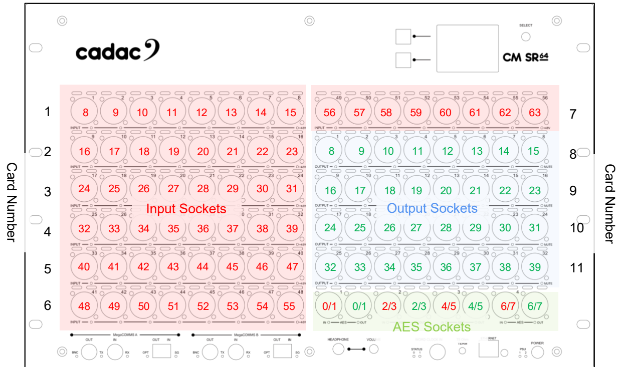
44: Cadac CM-SR64
